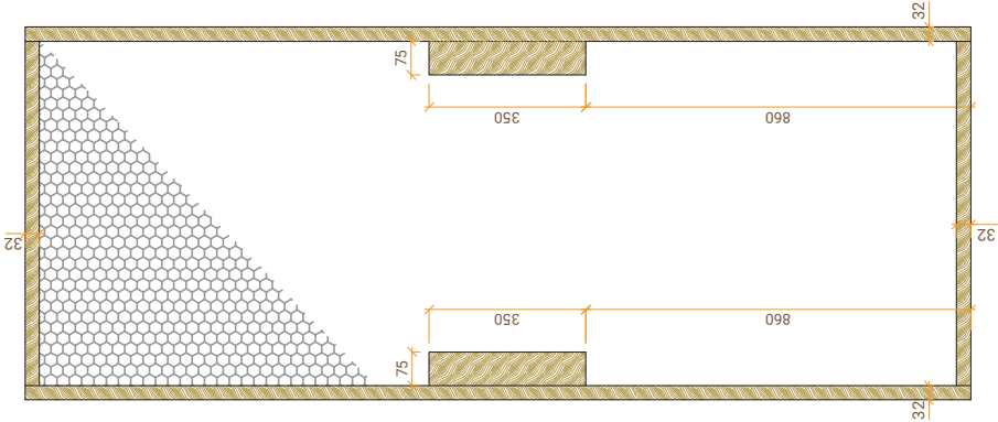
PROSPETTO PANNELLO PERSPECTIVE LEAF
